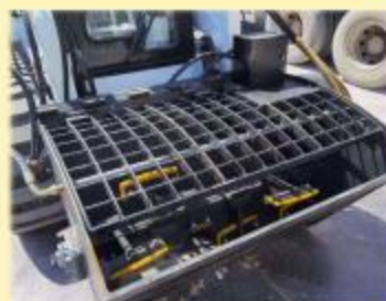
Bucket mixer
